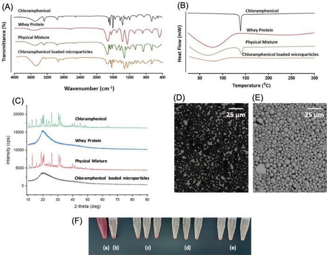
Figure 3. Representative image for FT-IR (A); DSC (B); XRD (C); light microscope (D) SEM (E) (The white scale exemplifies a length of 25 \mu\text{m} in each measurement), Hemolytic assay (F) of negative control (a), positive control (b), group of 500 ppm (c), group of 50 ppm (d), group of 5 ppm (e).
